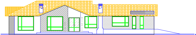
FACHADA PRINCIPAL
